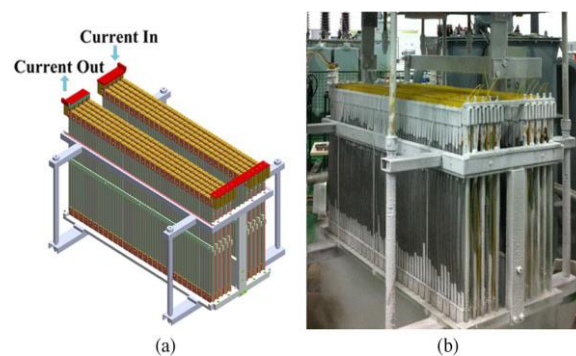
Figure 4. (a) Structure of the whole SFCL module (b) Real SFCL module
