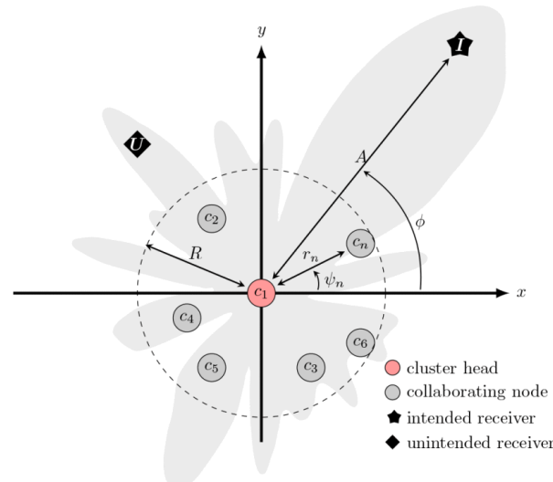
Figure 1. Randomly distributed sensor nodes perform CB through VAA [6]
