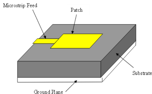
Figure 2. Patch antenna geometry
