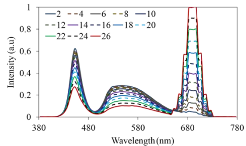
Figure 8. The emission spectra of 7700 K WLEDs as a function of (\text{Y,Gd})\text{BO}_3\text{:Eu} concentration
