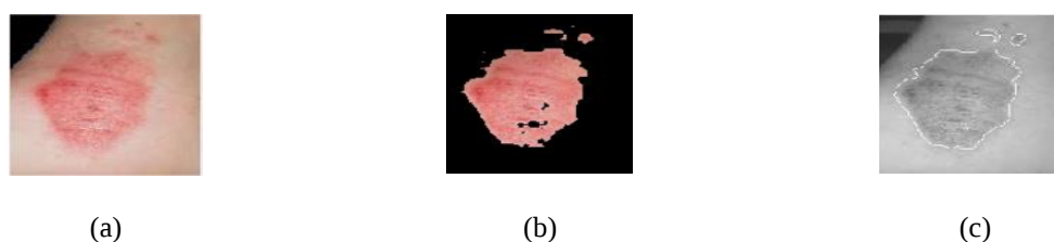
Figure 2. Diseases segmentation
