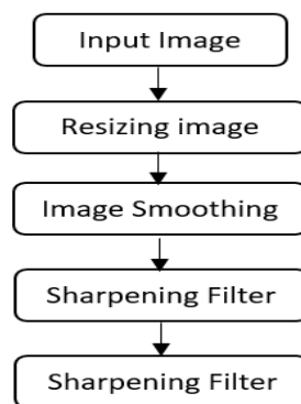
Figure 4. Enhancement process
