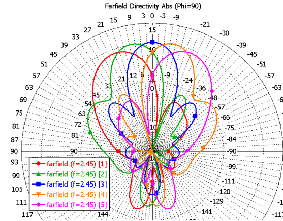
Figure 9. Radiation pattern beams for Rotman lens with antenna
