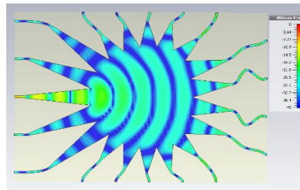
Figure 7. Electric field distribution through Rotman lens
