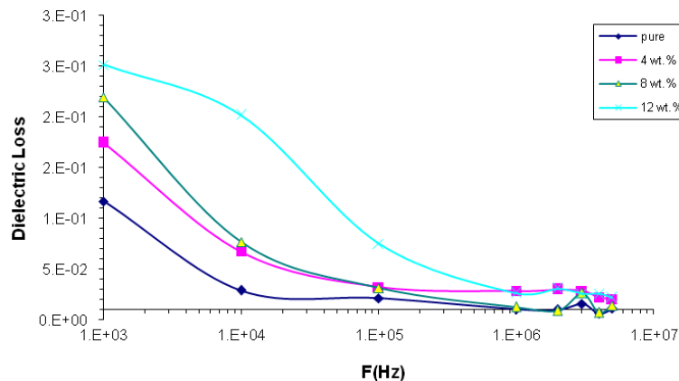
Figure 2. Variation of dielectric loss for (PS-CuO) nanocomposites with frequency
